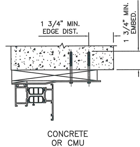
TYPICAL ANCHOR CONDITIONS WITH OPTIONAL WOOD BUCKS (1x MAX)
