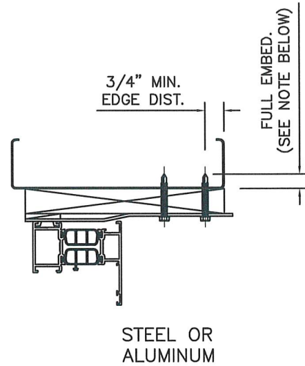
TYPICAL ANCHOR CONDITIONS WITH OPTIONAL WOOD BUCKS (1x MAX)
