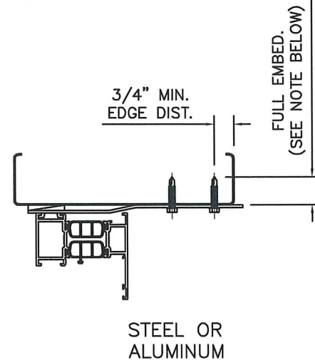
TYPICAL ANCHOR CONDITIONS (HEAD SHOWN. SILL AND JAMBS ARE SIMILAR)
